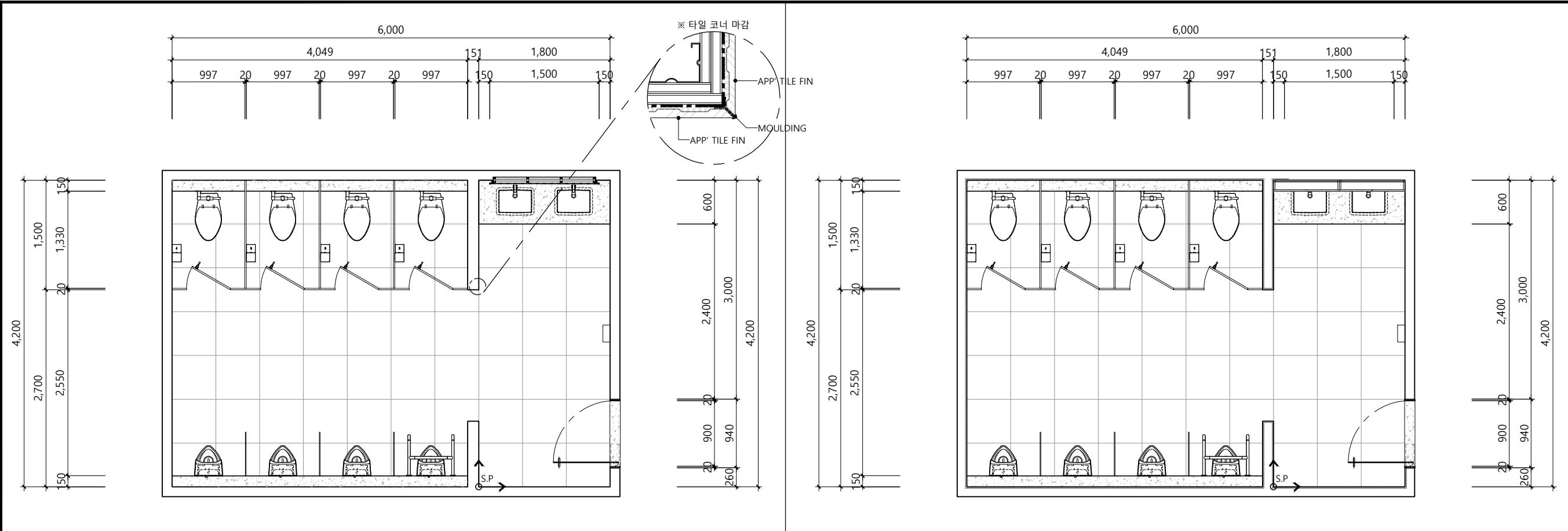
1 FLOOR PLAN_ALT.1 [고정형 거울] SCALE A1:1/30, A3:1/60 2 FLOOR PLAN_ALT.2 [가구형 거울] SCALE A1:1/30, A3:1/60
