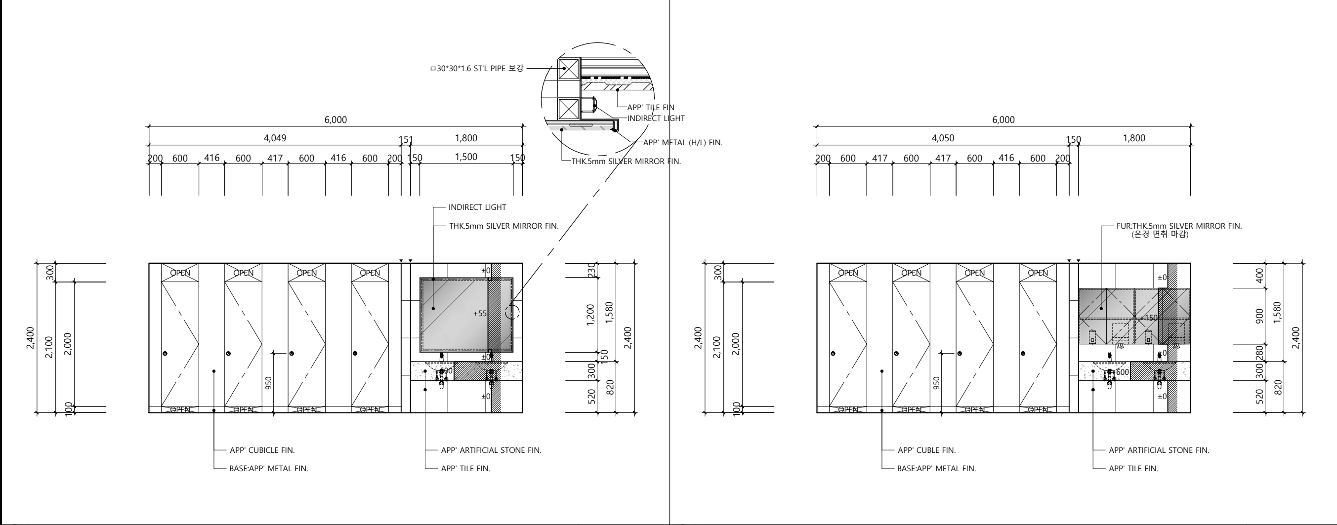
3 ELEVATION_ALT.1 [고정형 거울] SCALE A1:1/30, A3:1/60 4 ELEVATION_ALT.2 [가구형 거울] SCALE A1:1/30, A3:1/60
